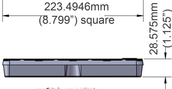
FRONT VIEW scale 1:3
